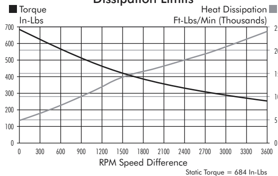
Torque and Heat Dissipation Limits
