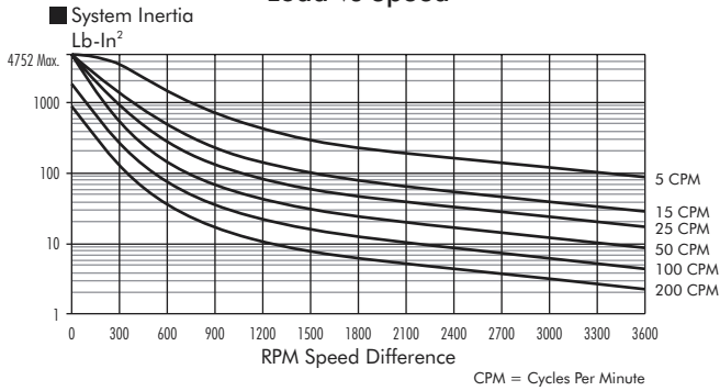
Cycle Rate Guide Load vs Speed
