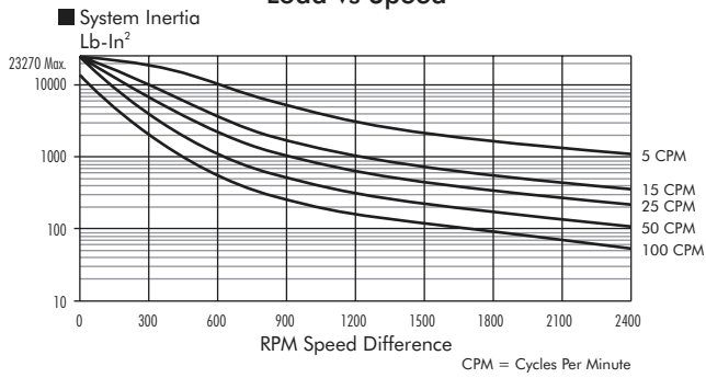
Cycle Rate Guide Load vs Speed
