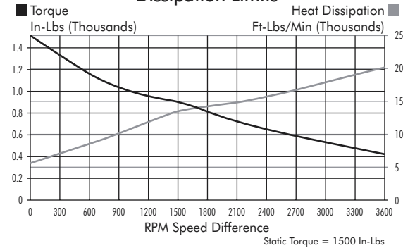
Torque and Heat Dissipation Limits
