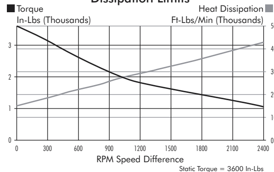
Torque and Heat Dissipation Limits
