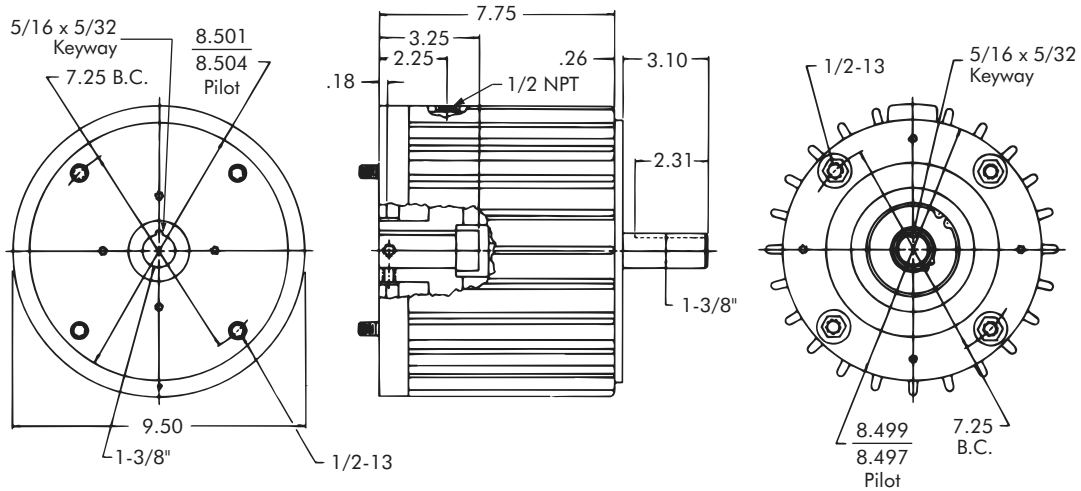
Clutch-Brake Module
